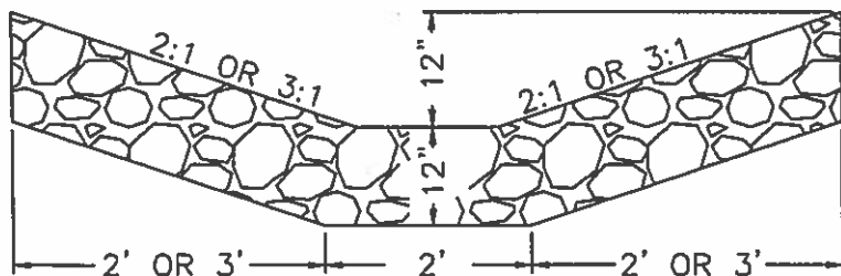
DETAIL OF AGGREGATE DITCH (SPECIAL)
