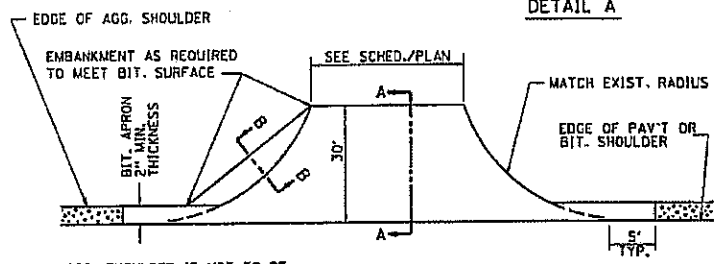
PLAN AT SIDE ROADS
