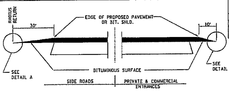
SECTION A-A DETAILS AT ENTRANCES & SIDE ROADS
