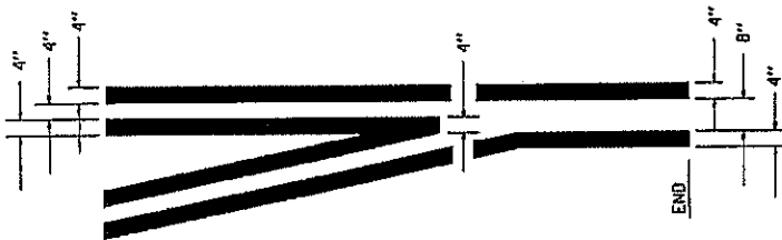
TYPICAL APPLICATION @ LEFT TURN LANES
