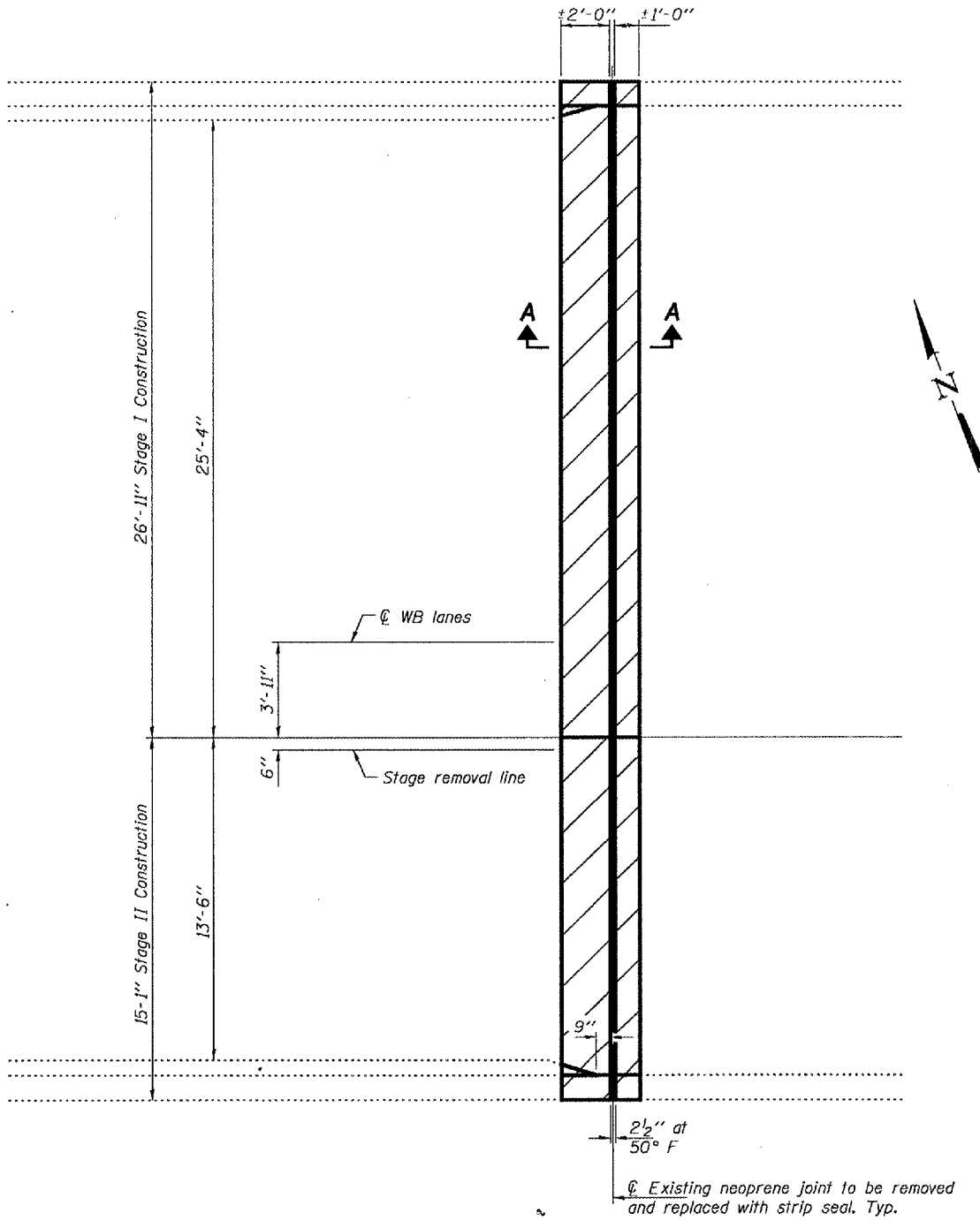
PLAN (Typ. at East Abutment)
