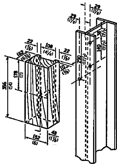
WOOD BLOCK-OUT AND STEEL POST DETAILS
