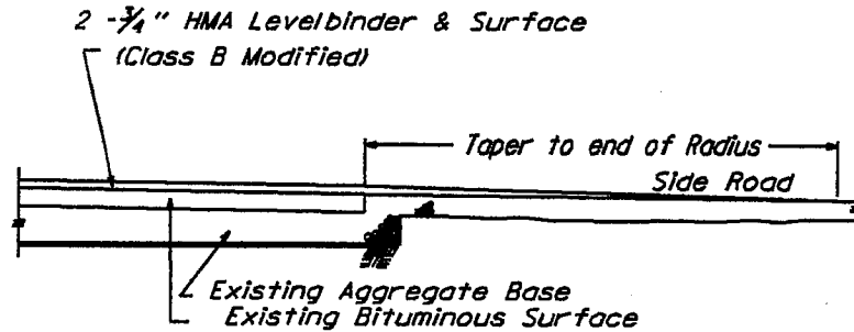
Side Road Taper Detail
