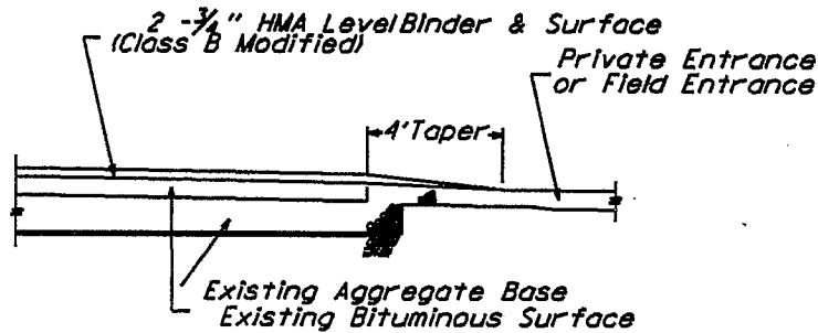
Entrance Taper Detail
