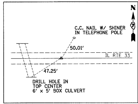
P.T. STA. 329+64.80 (MAG NAIL)
