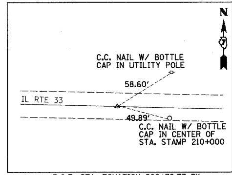
P.O.T. STA. EQUATION 209+78.77 BK 209+67.66 AH (MAG NAIL)
