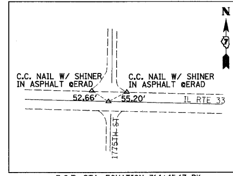
P.O.T. STA. EQUATION 314+45.17 BK 314+13.07 AH (MAG NAIL)
