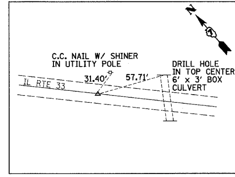
P.T. STA. EQUATION 355+20.31 BK 357+15.38 AH (MAG NAIL)
