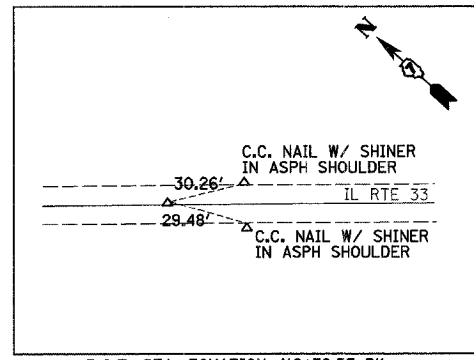
P.O.T. STA. EQUATION 412+78.37 BK 412+74.63 AH (MAG NAIL)
