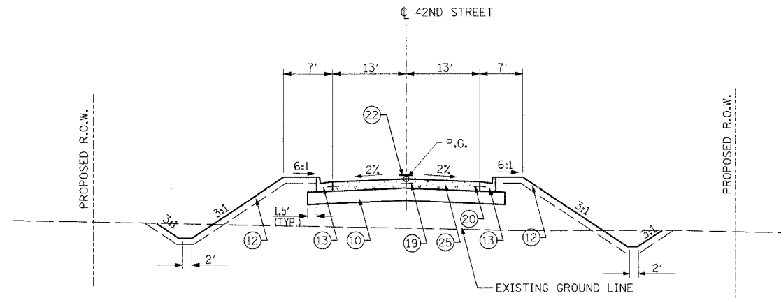
42ND STREET STA. 206+57.15 TO STA. 207+32.15
