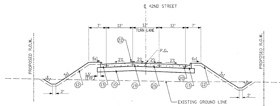
42ND STREET STA. 197+85.94 TO STA. 204+26.87 INTERSECTION OMISSION STA. 198+22.47 TO STA. 201+70.70 (VETERAN'S MEMORIAL DRIVE)
