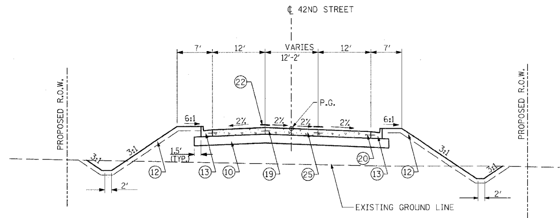
42ND STREET STA. 204+26.87 TO STA. 206+57.15
