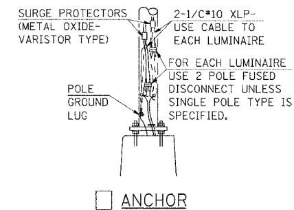
ANCHOR METAL OR CONCRETE DETAILS FOR UNDERGROUND DISTRIBUTION IF REQUIRED
