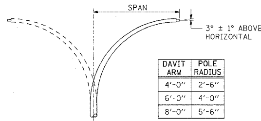
DAVIT ARM (AND OR) DAVIT ARM-TWIN
