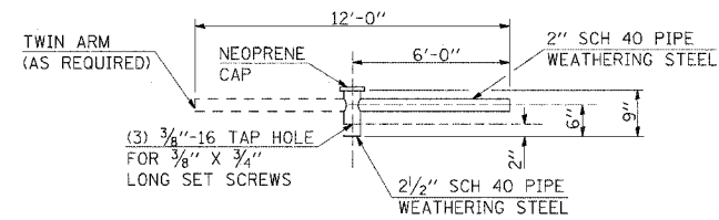
TENON MOUNT BRACKET ARM
