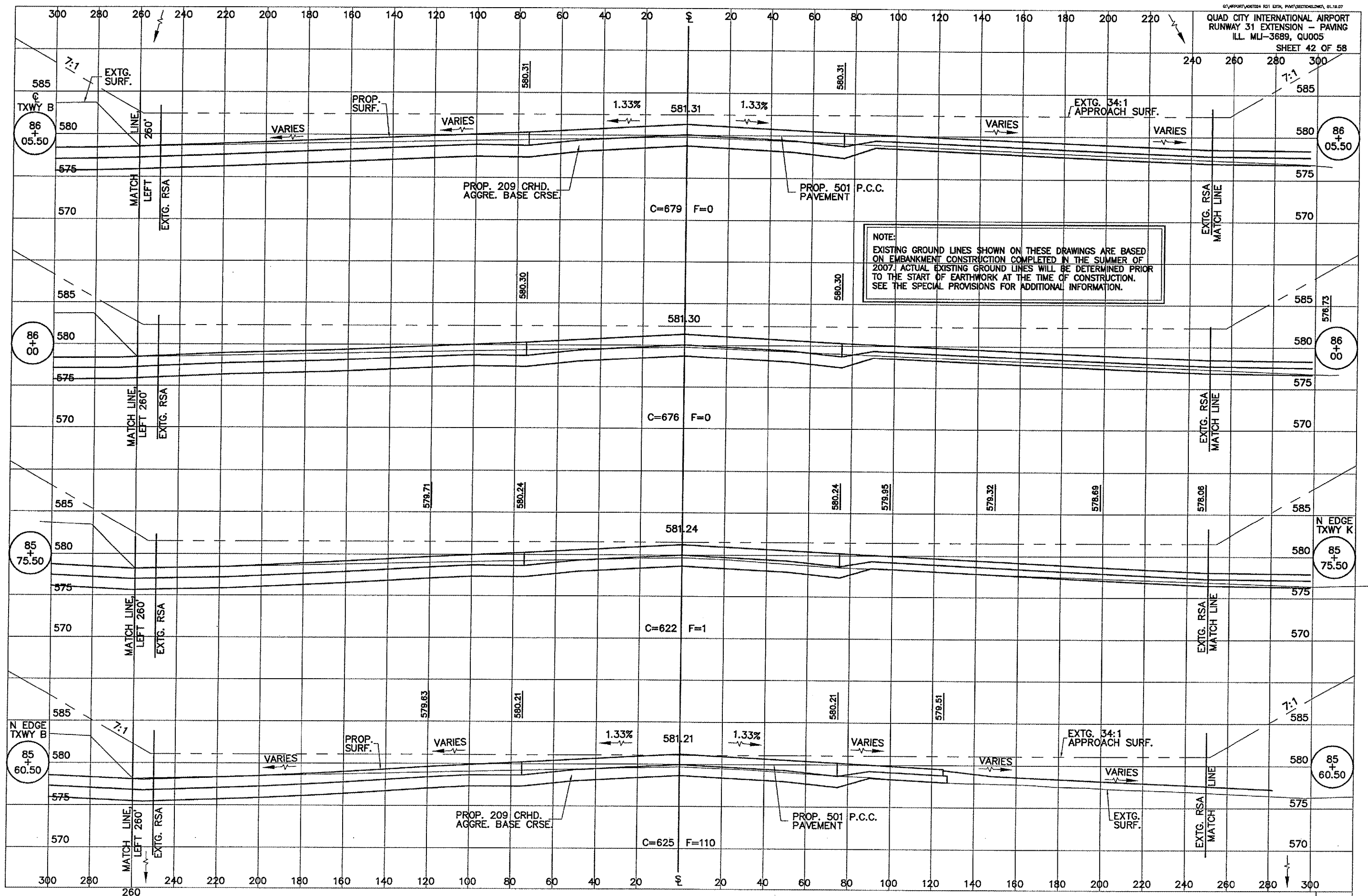
RUNWAY 31 CROSS SECTIONS, STA 85+60.50 TO STA 86+05.50 42/58
