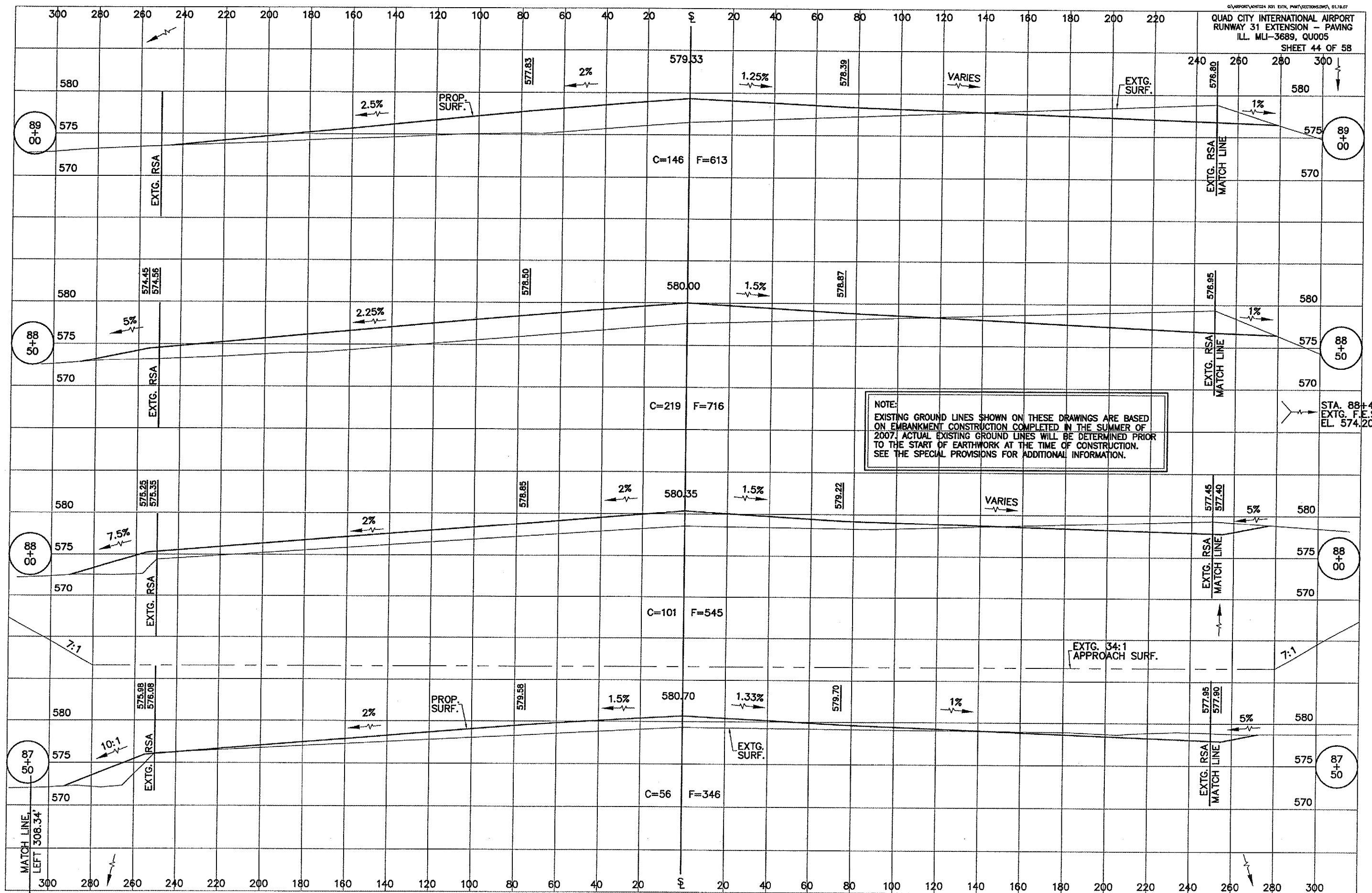
RUNWAY 31 CROSS SECTIONS, STA 87+50 TO STA 89+00
