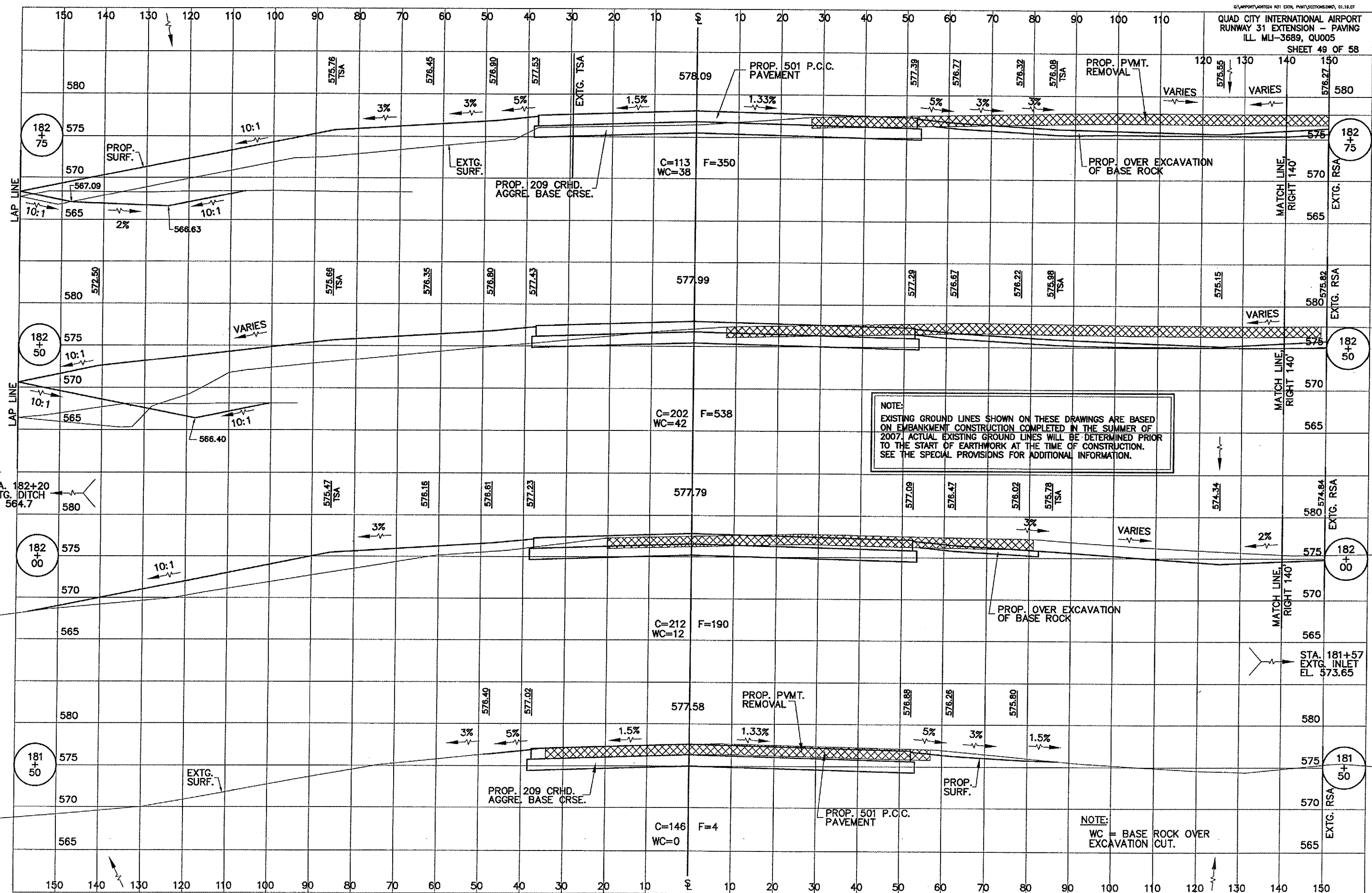
TAXIWAY B CROSS SECTIONS, STA 181+50 TO STA 182+75 49/58
