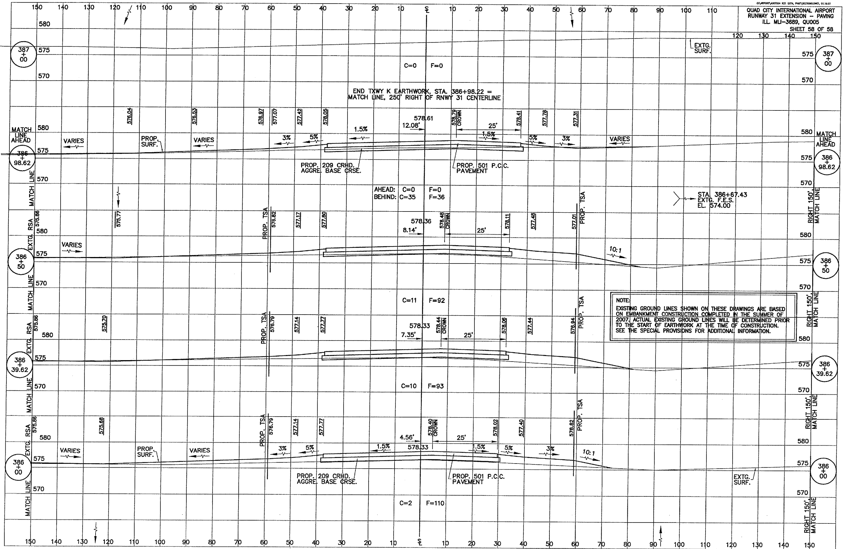
TAXIWAY K CROSS SECTIONS, STA 386+00 TO STA 387+00
