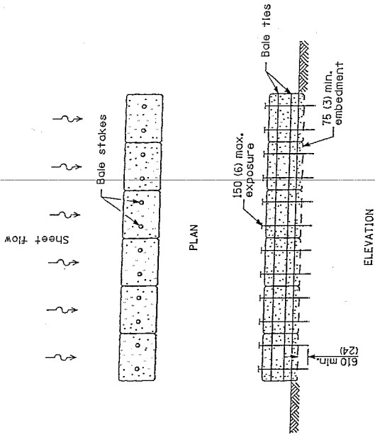
HAY OR STRAW BALES AS A PERIMETER EROSION BARRIER
