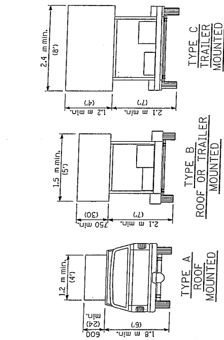
ARROW BOARDS
