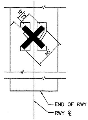
CLOSED RWY MARKER DETAIL N.T.S.
