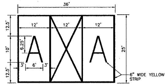
GAS TRUCK PARKING PAD PAINT DETAIL ~ N.T.S. ~
