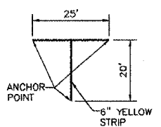
TIE DOWN PAINT DETAIL ~ N.T.S. ~
