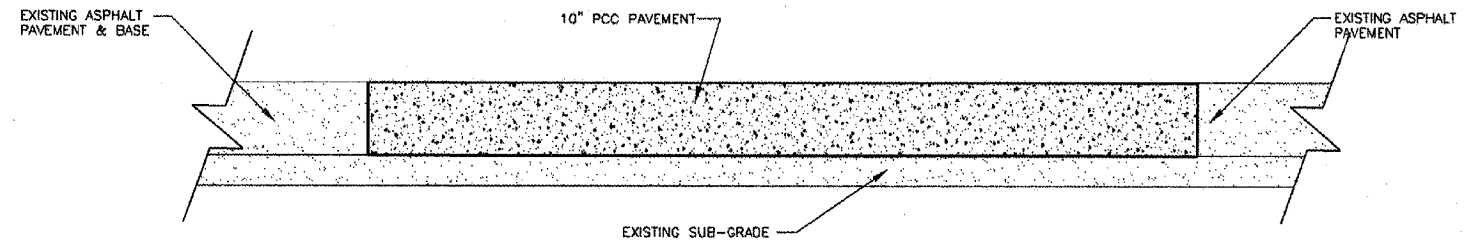
TYPICAL SECTION FOR FUEL TRUCK PAD GA RAMP 10\"/>
