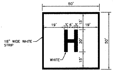
HELICOPTER PAD PAINT DETAIL ~ N.T.S. ~
