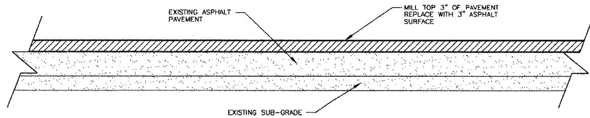
TYPICAL SECTION FOR AREAS TO BE MILLED GA RAMP 3\"/>
