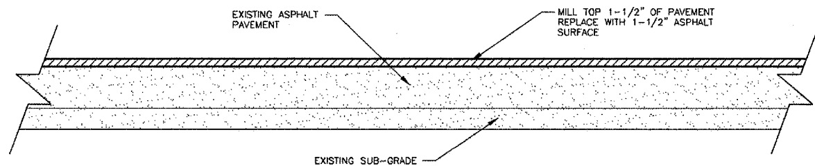
TYPICAL SECTION FOR AREAS TO BE MILLED GA RAMP 1-1/2\"/>
