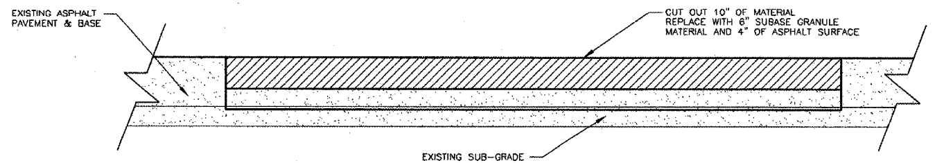
TYPICAL SECTION FOR AREAS TO BE PATCHED GA RAMP 6\"/>
