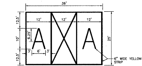
GAS TRUCK PARKING PAD PAINT DETAIL ~ N.T.S. ~
