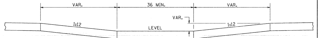
SECTION B-B
