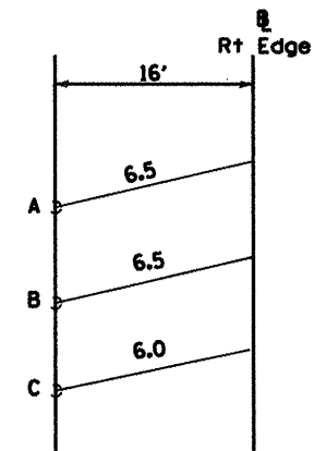
AXIS OF ROTATION & PROFILE GRADE LINE
