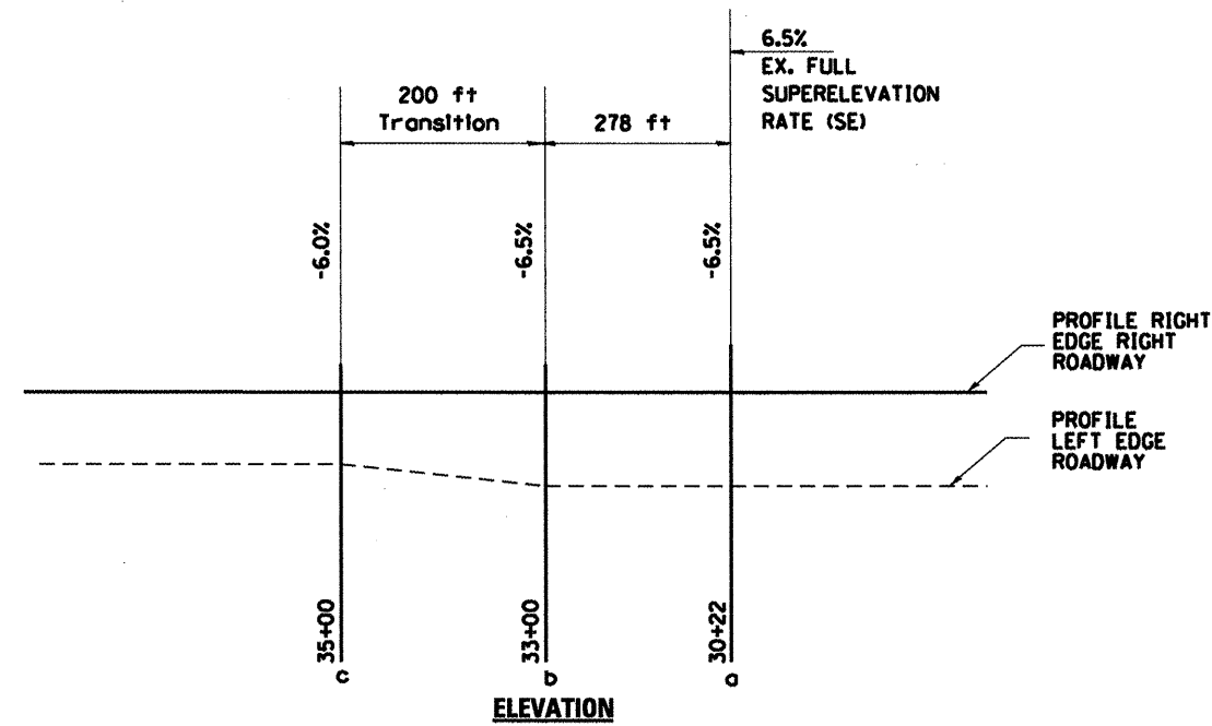
AXIS OF ROTATION & PROFILE GRADE LINE
