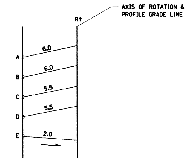
CROSS SECTIONS SUPERELEVATION DETAILS
