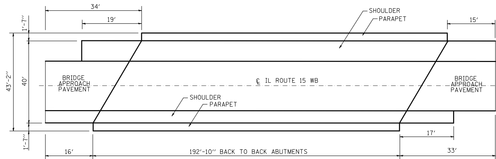
PLAN VIEW
