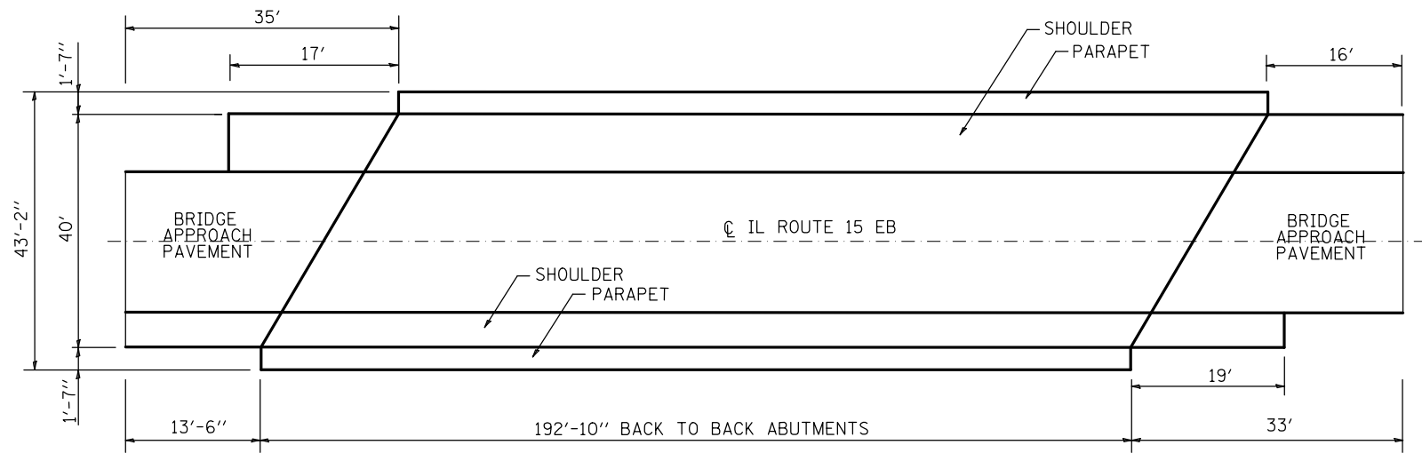
PLAN VIEW
