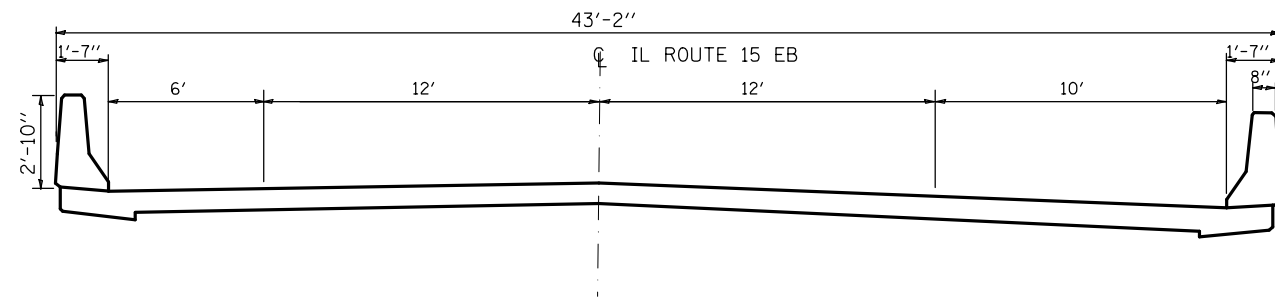
TYPICAL SECTION
