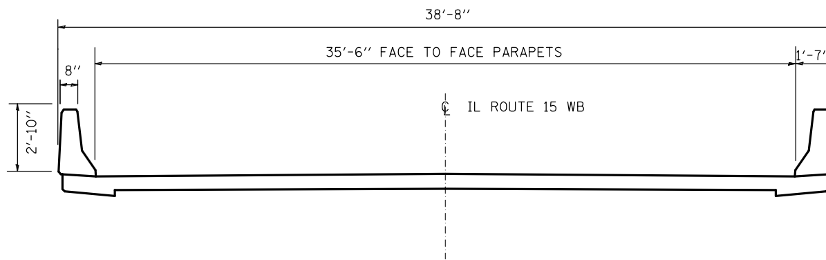
TYPICAL SECTION
