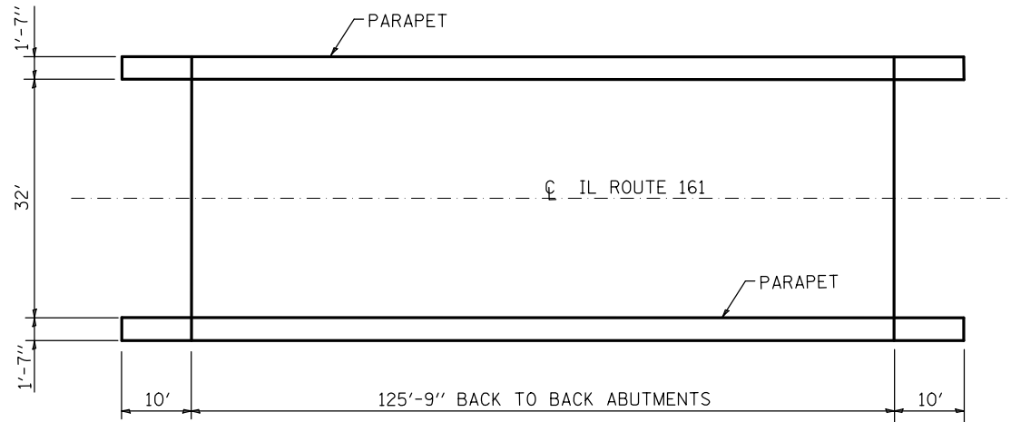
PLAN VIEW
