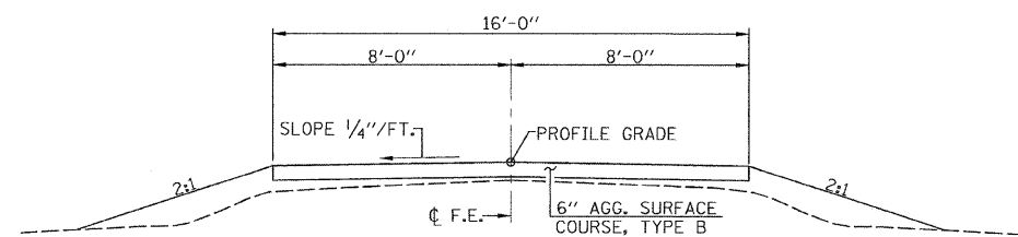
TYPICAL FIELD ENTRANCE
