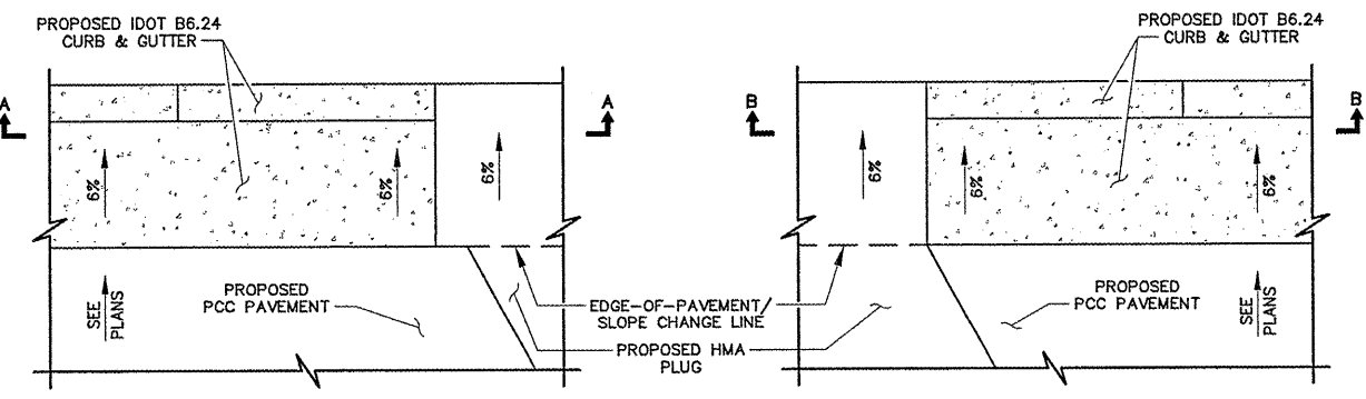
CURB HEIGHT TRANSITION DETAIL N.T.S.
