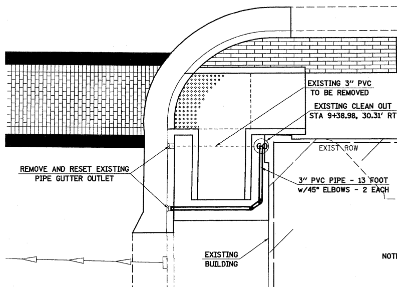
CURB RAMP AND CROSS SIDEWALK DRAIN DETAIL E. FERGUSON AT N. WHITELAW AVE.
