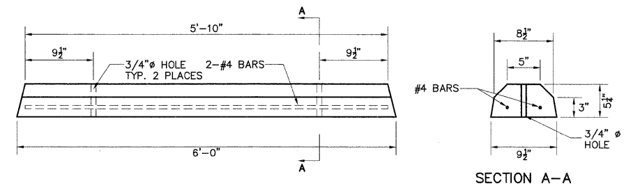
CONCRETE PARKING BLOCK DETAIL NOT TO SCALE
