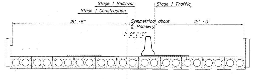
CROSS SECTION (Looking East)
