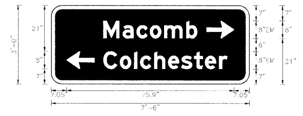
SIGN DETAIL 1:20
