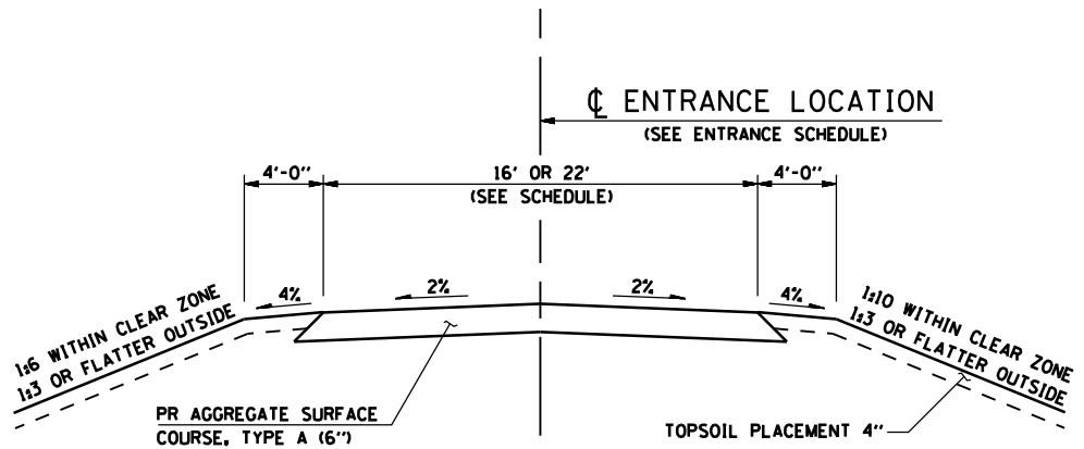
TYPICAL SECTION - (PE) OR (FE) (SEE SCHEDULE FOR LOCATIONS)
