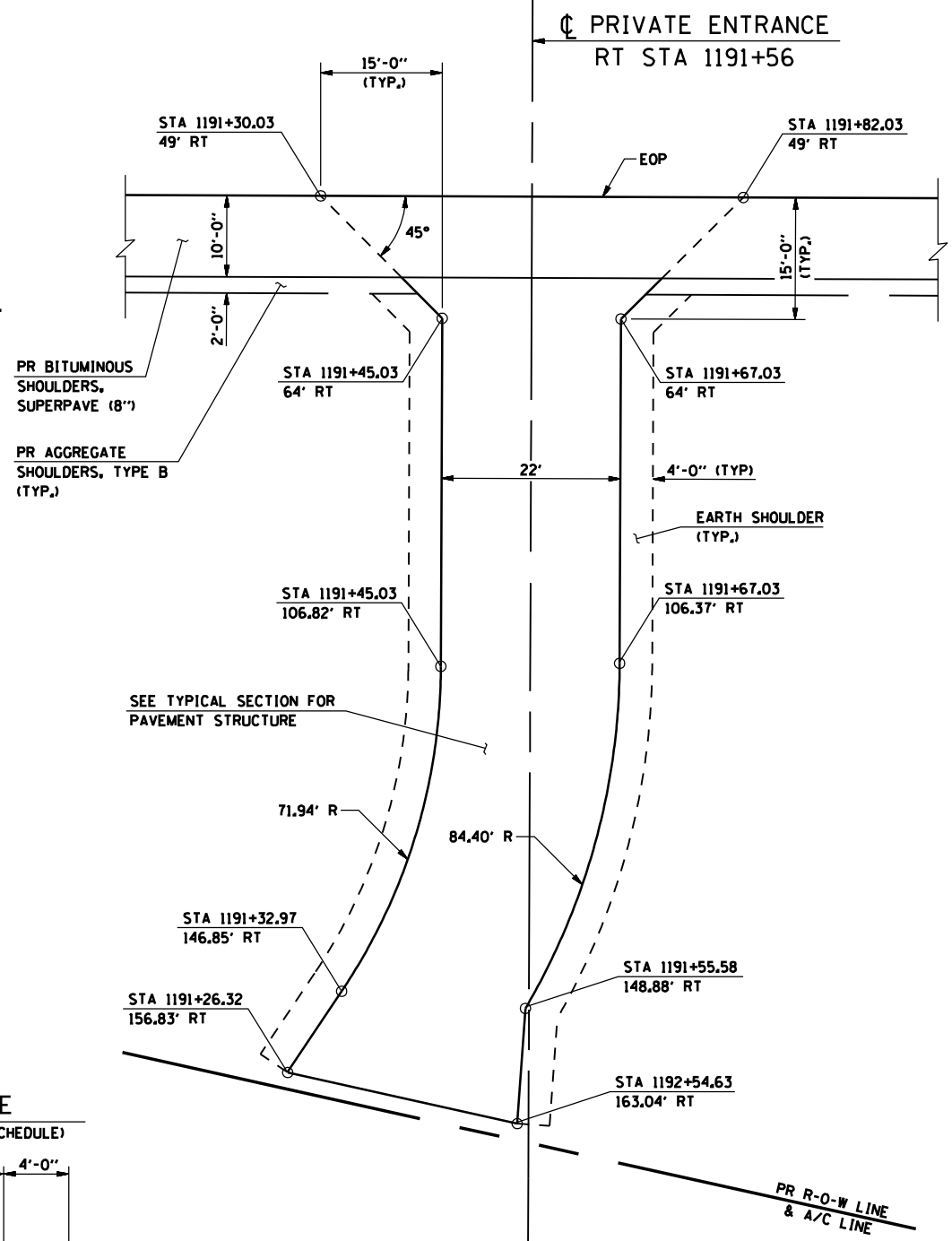
PLAN - PRIVATE ENTRANCE (PE) RT STA 1191+56.00 (IL RTE 336)
