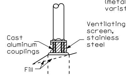
BREAKAWAY COUPLING
