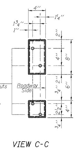
END OF RAIL DETAILS
