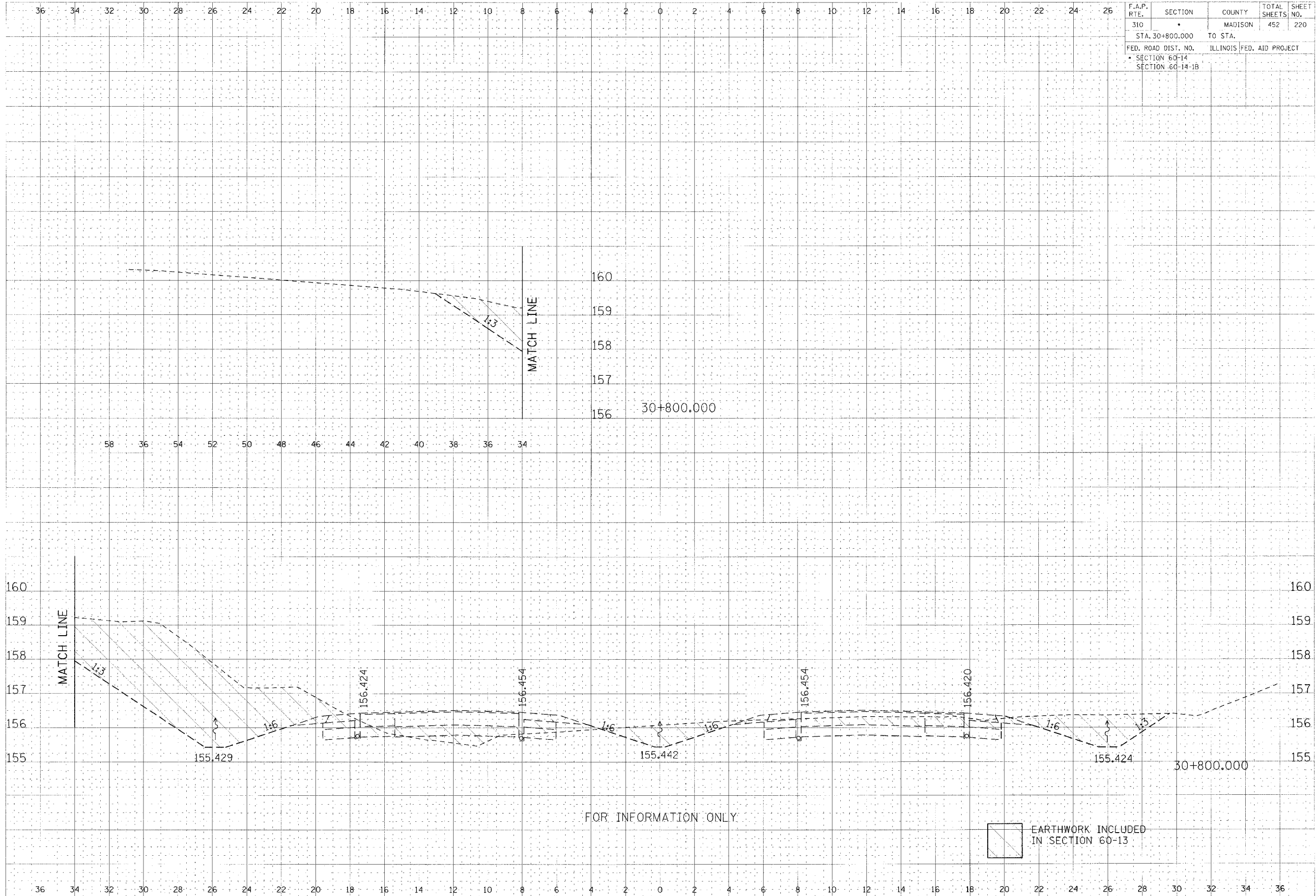
CROSS SECTION, FAP ROUTE 310, STA 30+800.000
