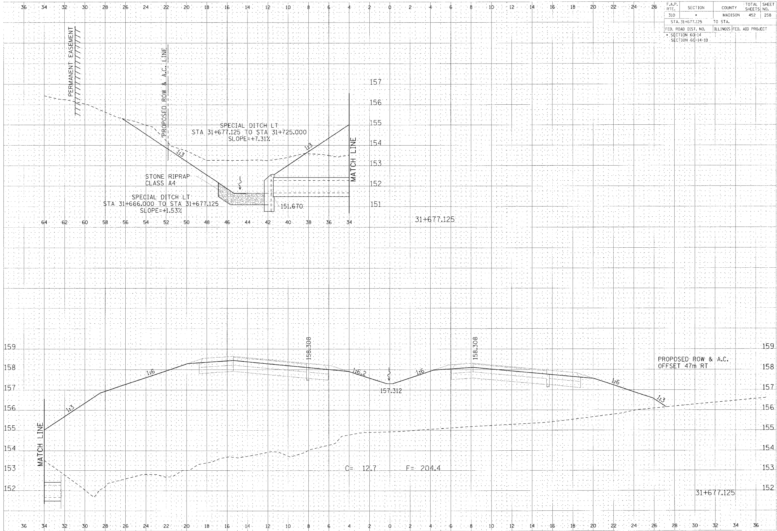
CROSS SECTION, FAP ROUTE 310, STA 31+677.125
