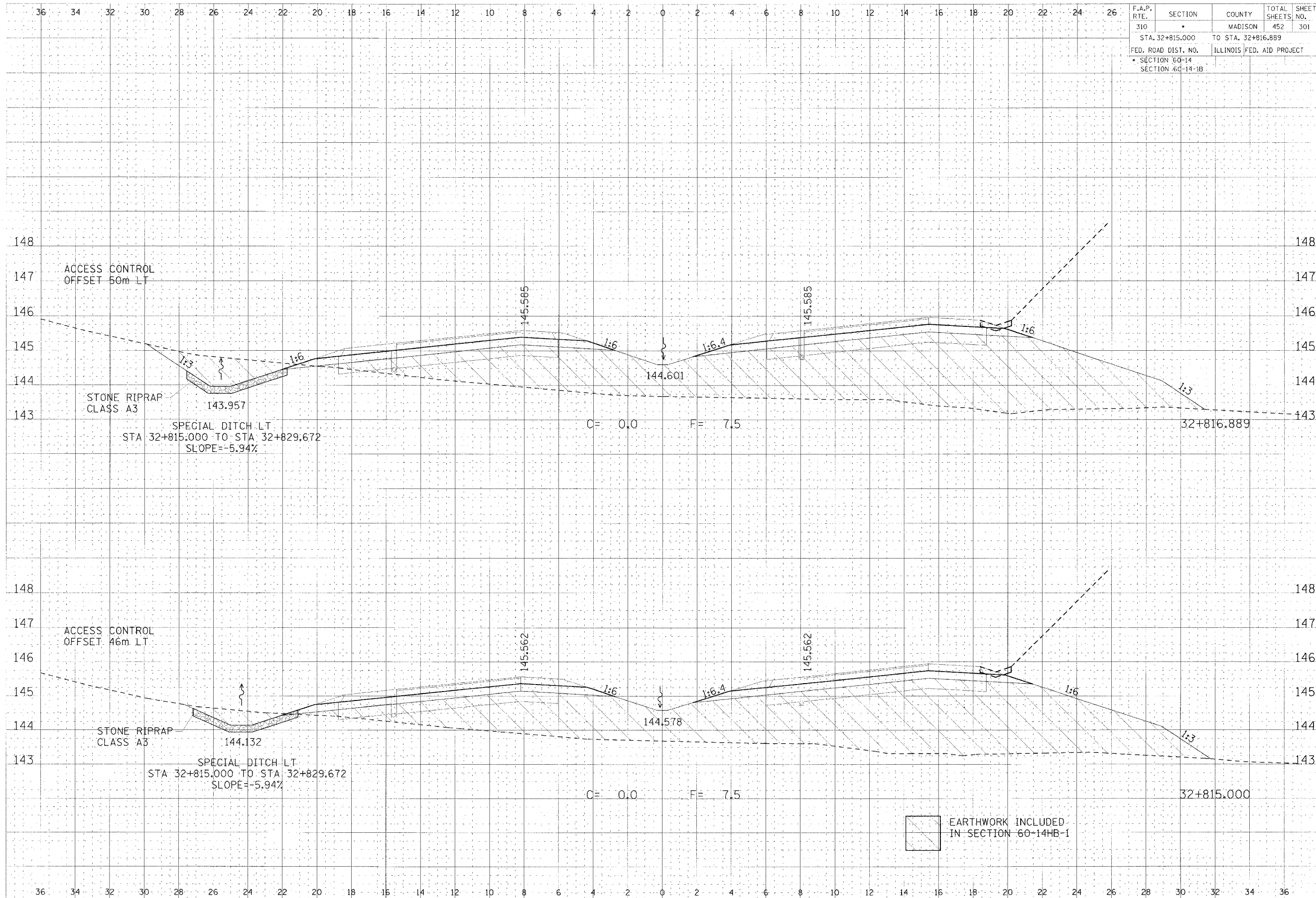
CROSS SECTION, FAP ROUTE 310, STA 32+815.000 TO STA 32+816.889
