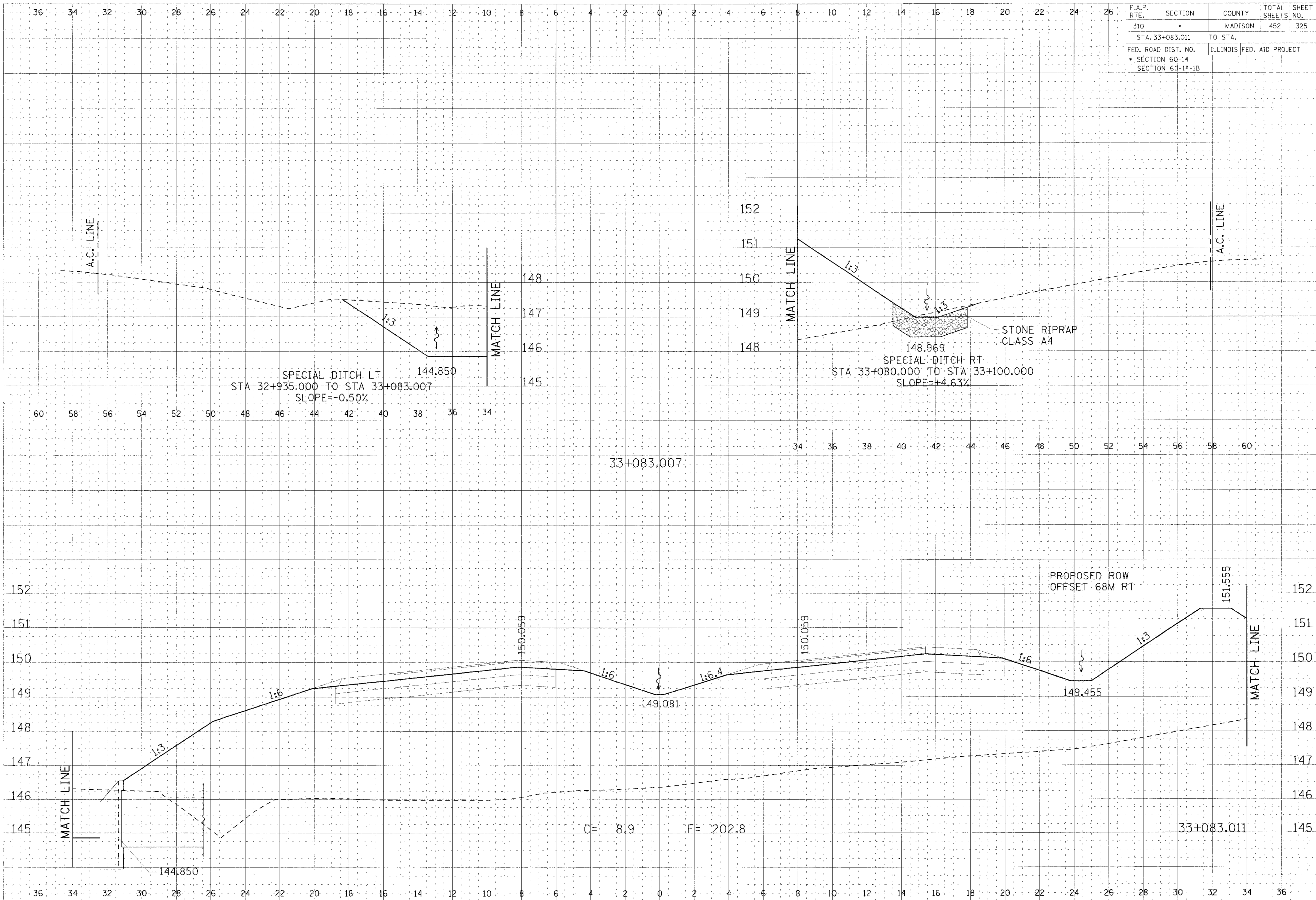
CROSS SECTION, FAP ROUTE 310, STA 33+083.011
