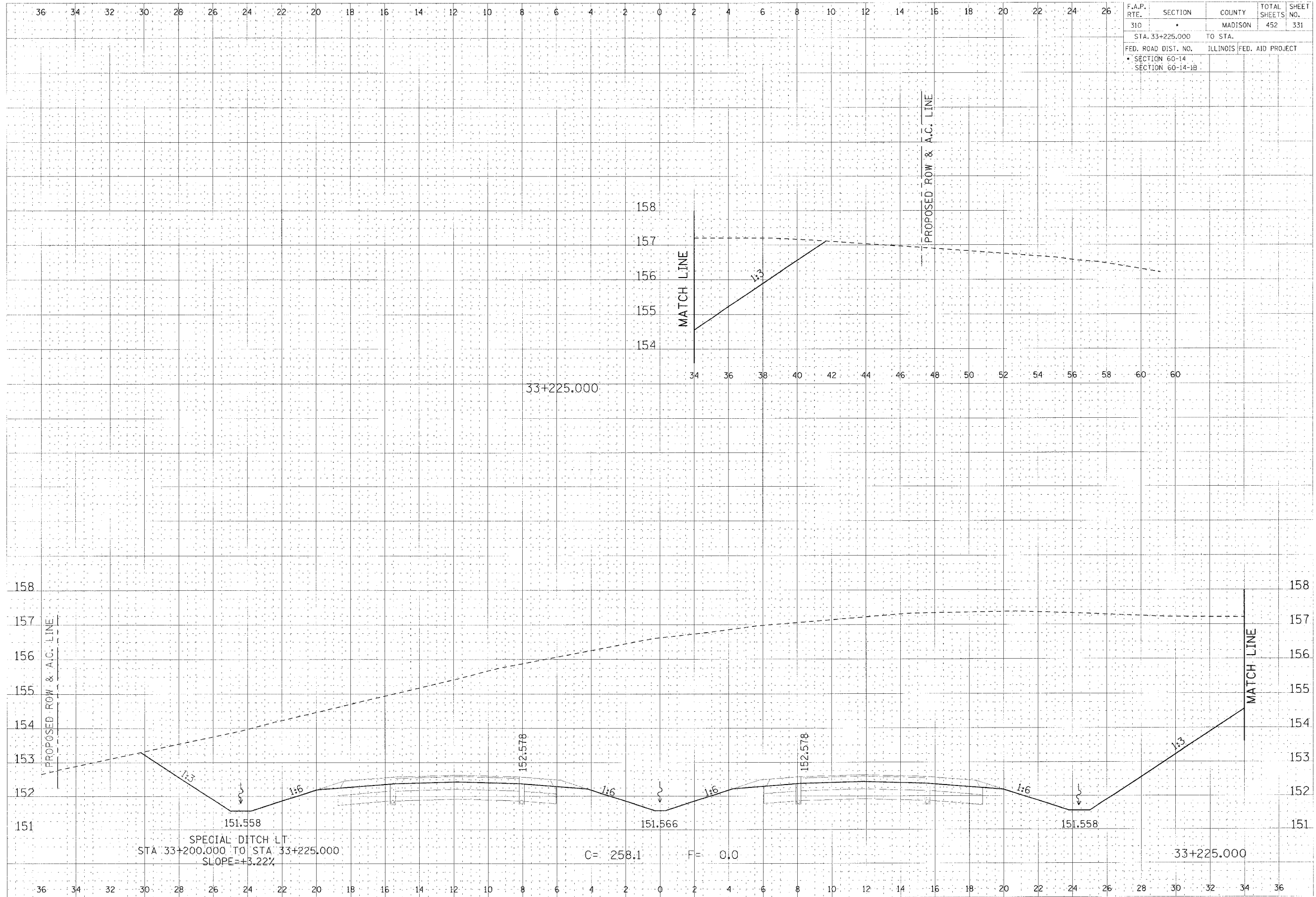
CROSS SECTION, FAP ROUTE 310, STA 33+225.000
