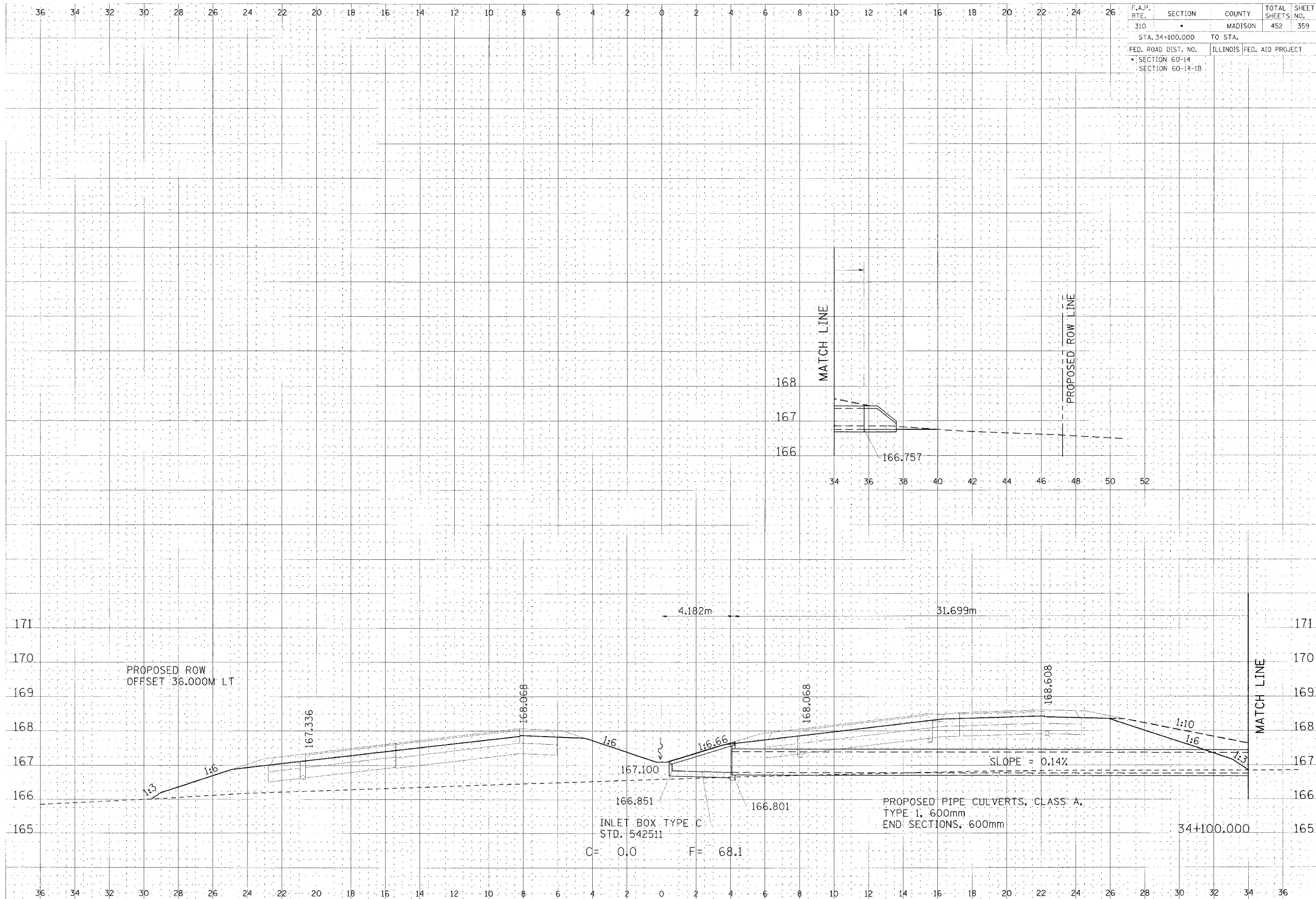
CROSS SECTION, FAP ROUTE 310, STA 34+100.000
