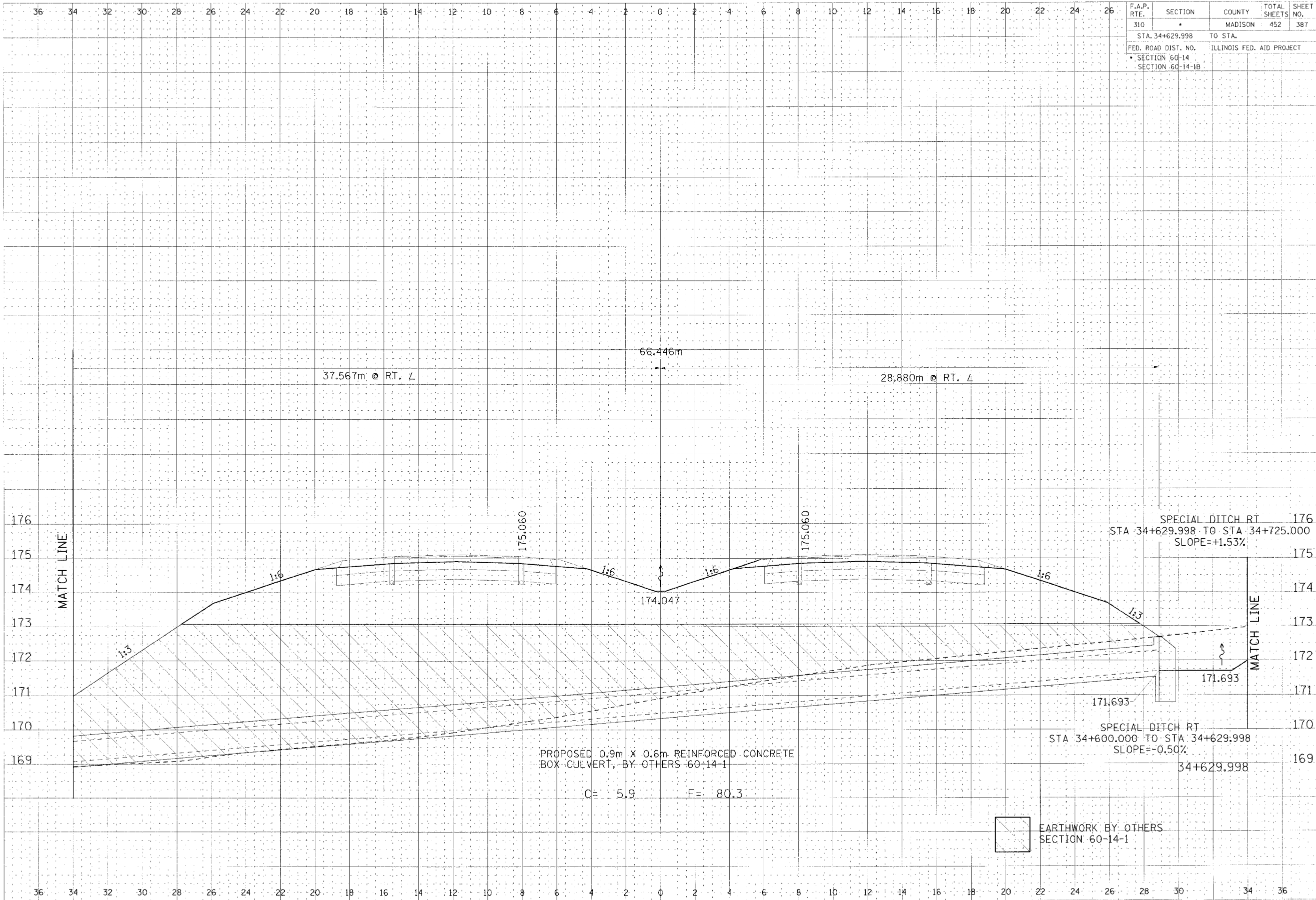
CROSS SECTION, MAINLINE, STA 34+629.998
