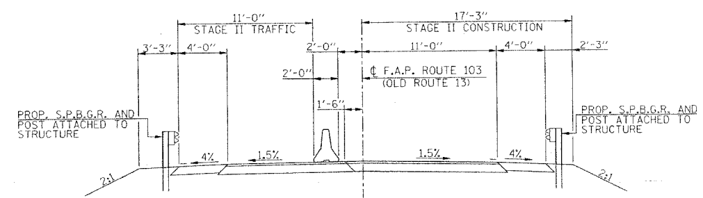
STAGE II TRAFFIC OVER PROPOSED CULVERT (LOOKING UPSTATION)
