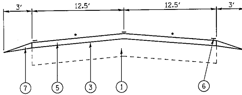
TYPICAL SECTION STA. 1245+20 TO STA. 1293+72
