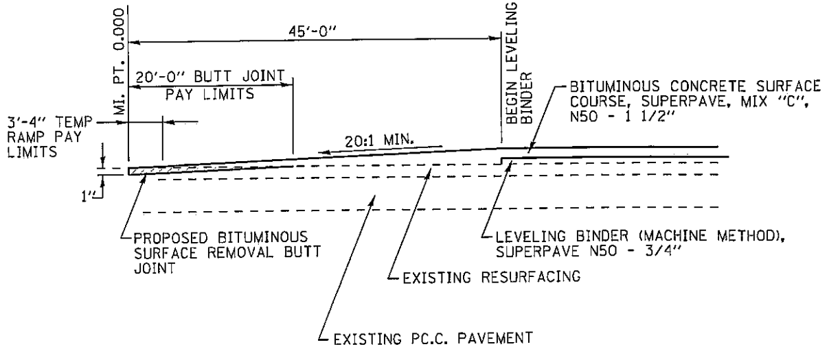
BUTT JOINT DETAIL MILE PT. 0.000
