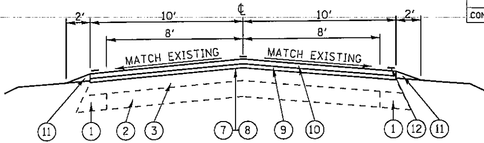
TYPICAL SECTION MILE PT. 0.000 TO 0.554 EXCLUDING STRUCTURE AT MILE PT. 0.220 (SEE TYPICAL BELOW)
