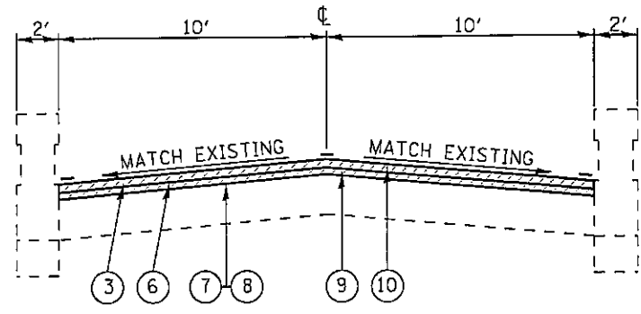
STRUCTURE NO. 003-0038 MILE PT. 0.220
