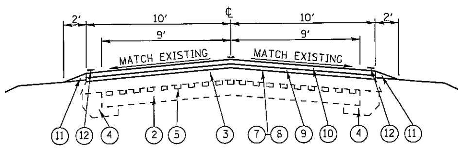
TYPICAL SECTION MILE PT. 0.554 TO 1.038
