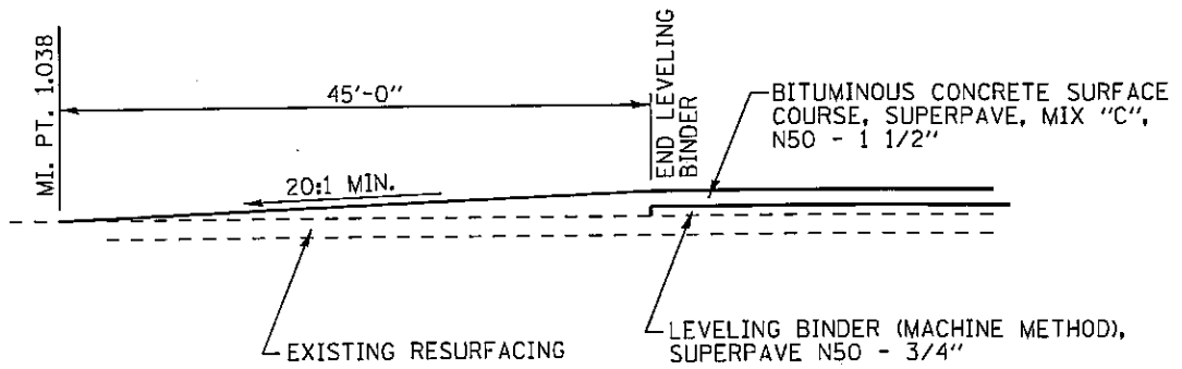
FEATHER EDGE DETAIL MILE PT. 1.038
