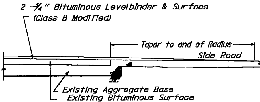
Side Road Taper Detail
