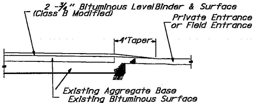
Entrance Taper Detail
