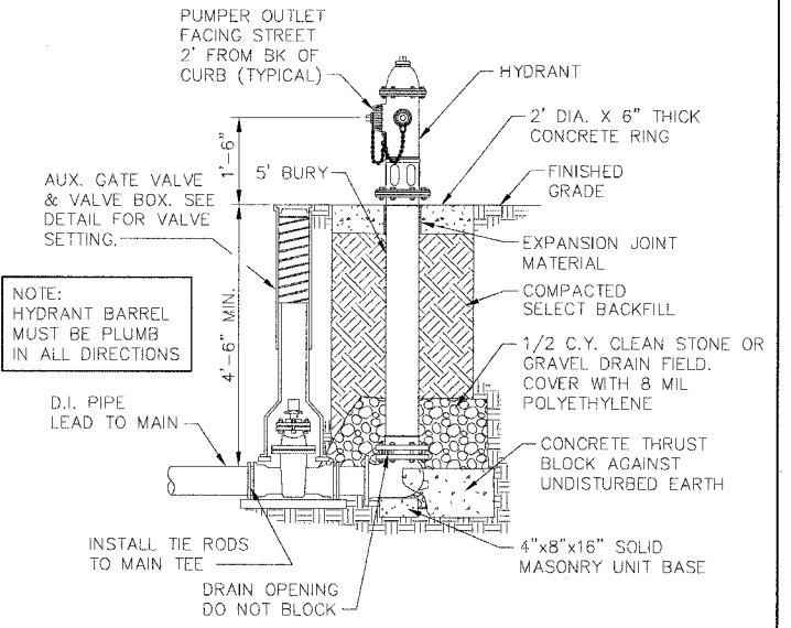
CITY OF QUINCY FIRE HYDRANT INSTALLATION NTS
