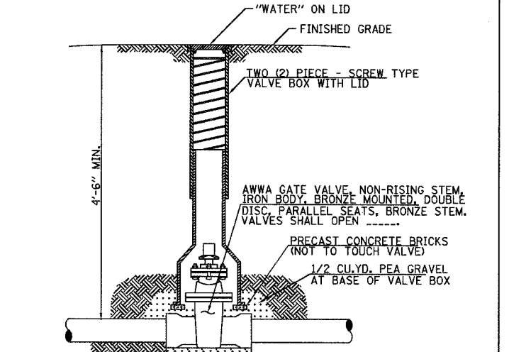
VALVE SETTING NOT TO SCALE
