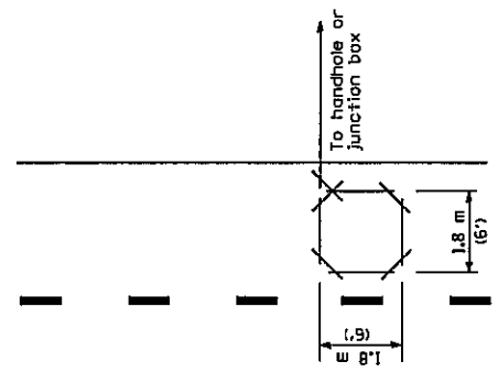
FOR POINT DETECTION SHORT LOOP
