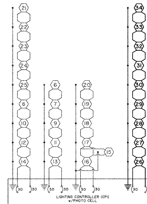
WIRING DIAGRAM
