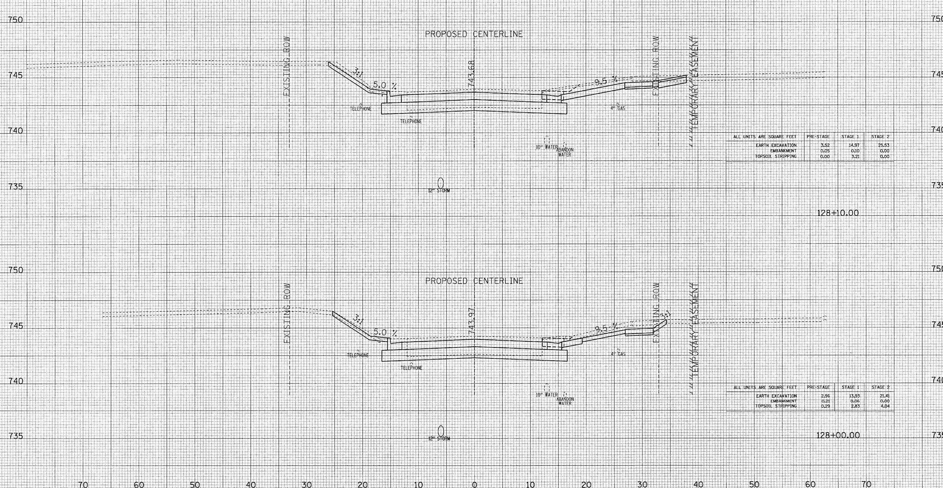
MAPLE AVENUE CROSS SECTIONS
