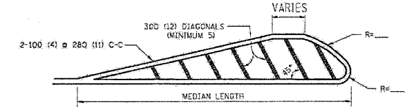
1.2 m (4') WIDE MEDIANS ONLY
