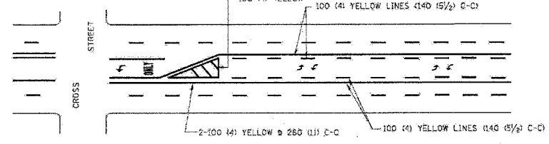
MEDIANS OVER 1.2 m (4') WIDE
