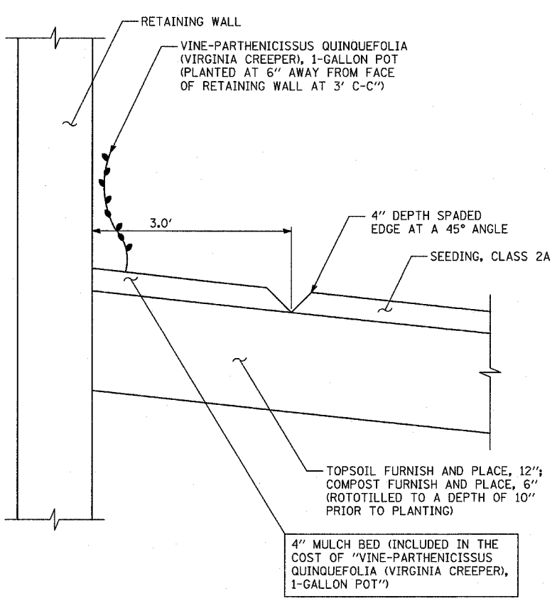
VINE PLANTING DETAIL
