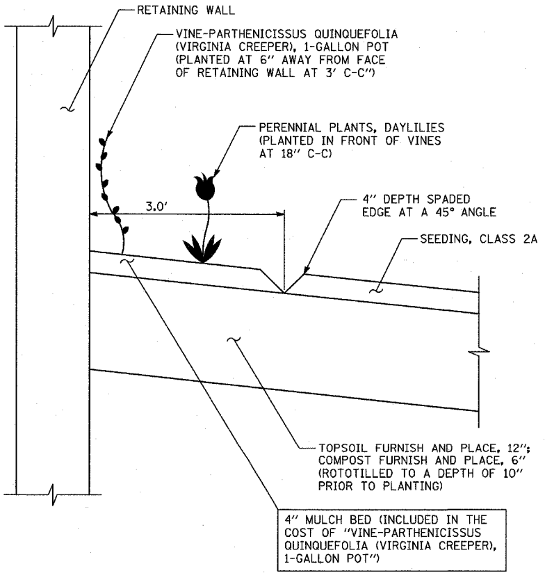
VINE AND DAYLILY PLANTING DETAIL
