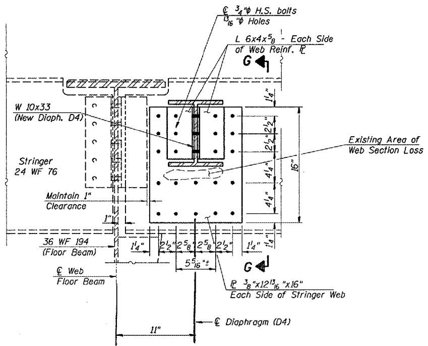
2 - STRINGER WEB REPAIR Looking West @ Panel Pl. L15 - Stringer Lines ③ & ④
