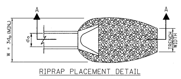
TYPE "A" RIPRAP DETAIL FOR DISCHARGE INTO WELL DEFINED CHANNEL
