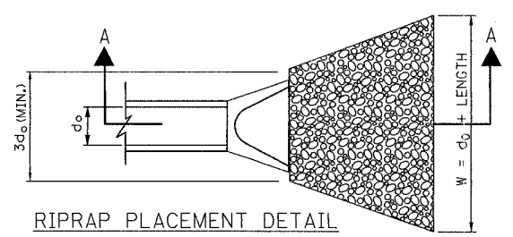
TYPE "B" RIPRAP DETAIL FOR DISCHARGE TO FLAT AREA WITH NO DEFINED CHANNEL
